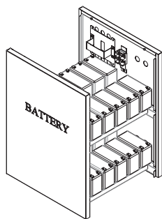
12pcs Batteries 6AH/7AH/9AH 151 × 65 × 100 (L × W × H)
