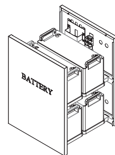
4pcs Batteries 100AH/120AH 407 × 174 × 236 (L × W × H)
