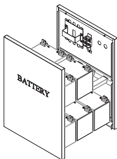
10pcs Batteries 33AH 196 × 131 × 156 (L × W × H)
