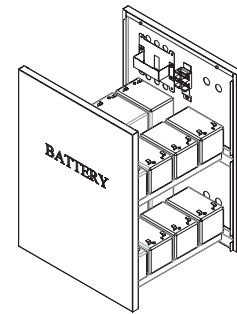
16pcs Batteries 12AH 151 × 98 × 100 (L × W × H)
