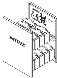
18pcs Batteries 15AH/20AH/22AH 181 × 77 × 167 (L × W × H)
