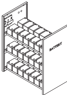
42pcs Batteries 12AH 151 × 98 × 100 (L × W × H)
