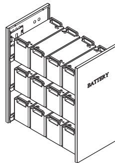
12pcs Batteries 100AH/120AH 407 × 174 × 236 (L × W × H)
