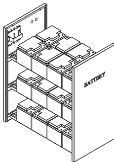
24pcs Batteries 38AH/45AH 198 × 166 × 170 (L × W × H)
